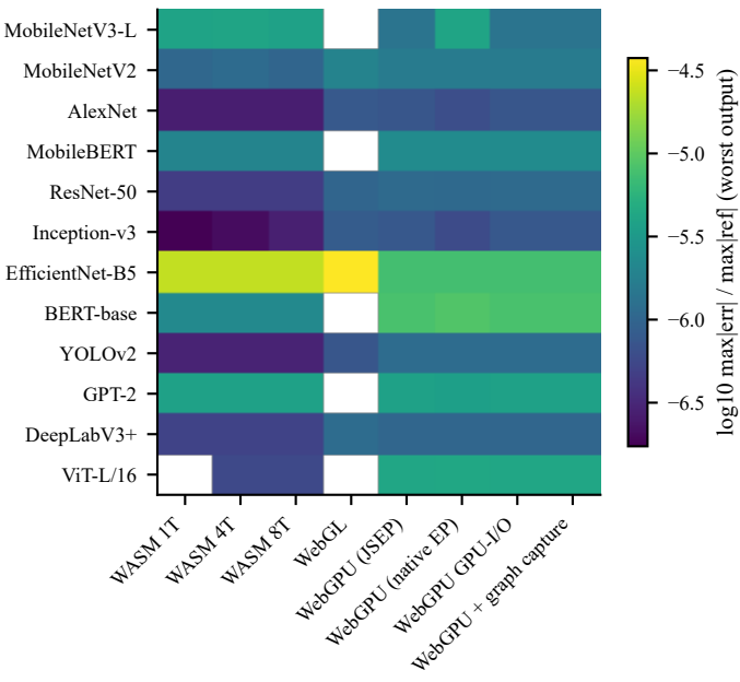
Deviation from native ONNX Runtime (CPU)
