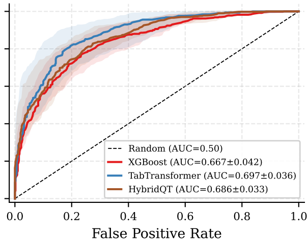
FHS Dataset (Framingham, n=4,240)
