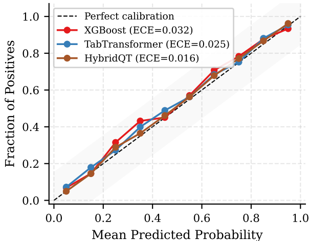
Reliability Diagram (CKD)
