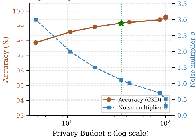
Privacy-Utility Tradeoff (DP-SGD, \delta=1e-5 )
