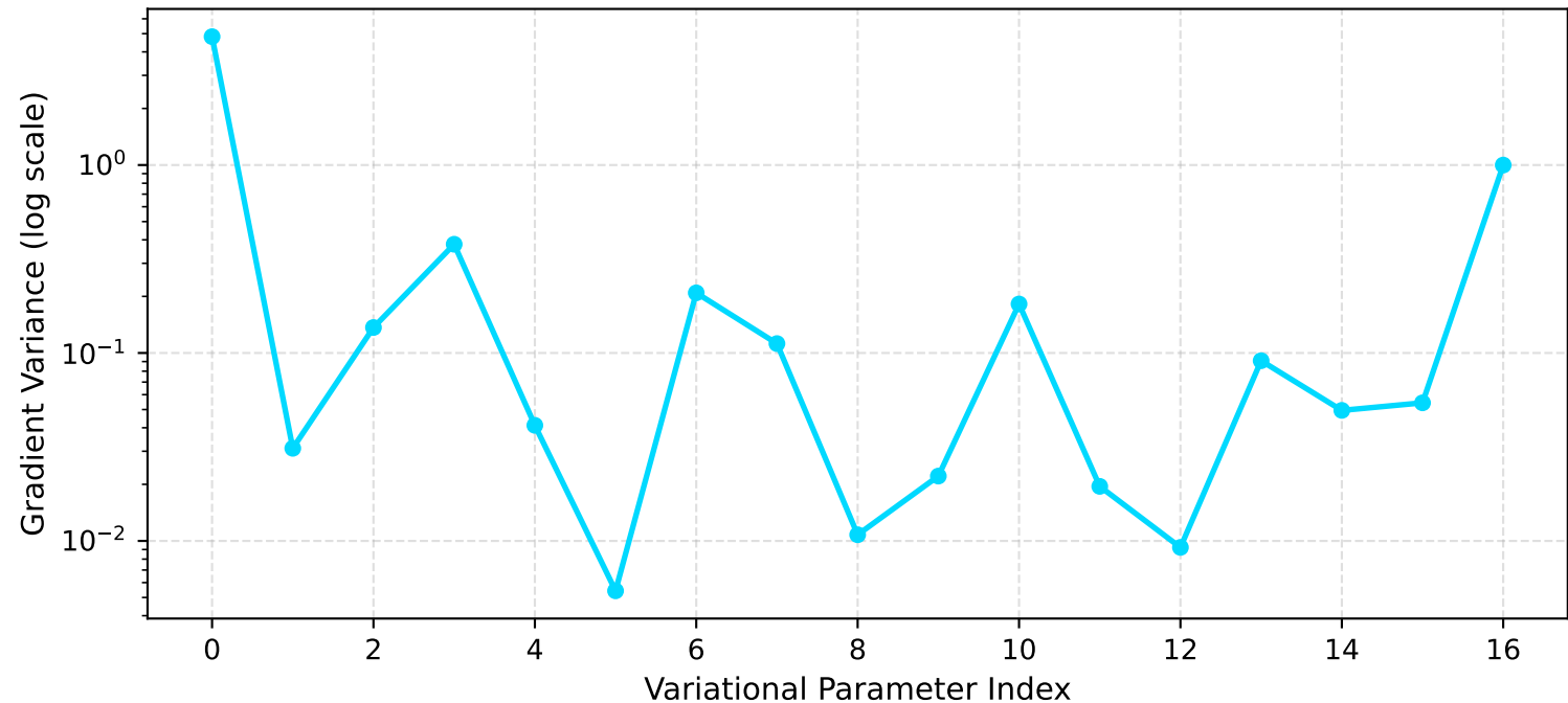
Barren Plateau Analysis — Gradient Variance vs Parameter Index
