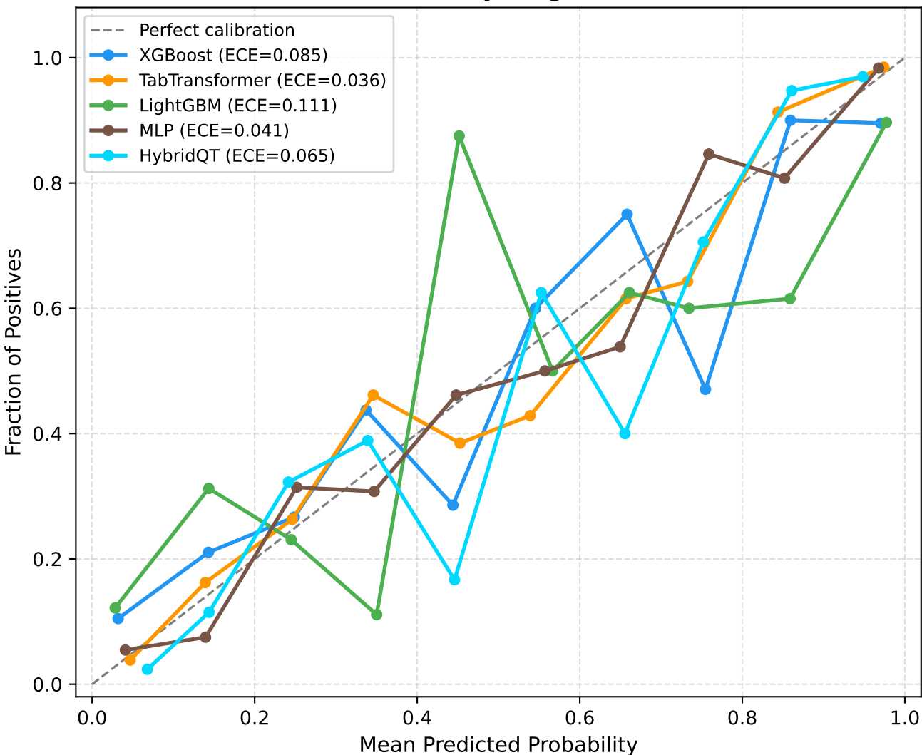
Calibration Reliability Diagram — Cleveland
