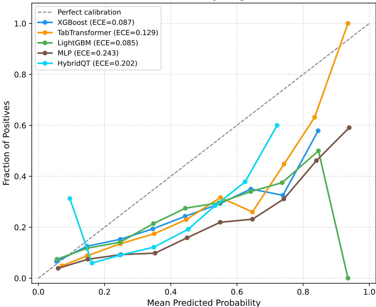
Calibration Reliability Diagram — FHS
