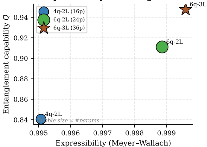
Expressibility vs Entanglement
