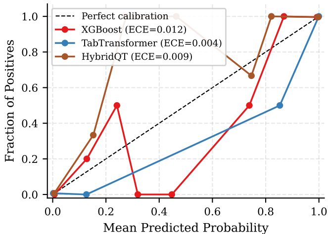
Reliability Diagram (CKD)
