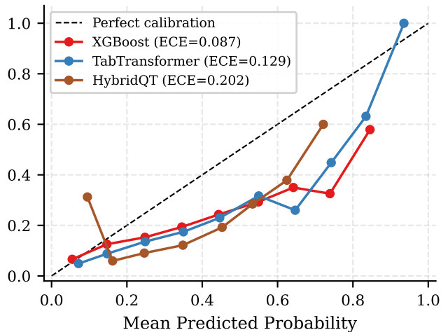
Reliability Diagram (FHS)
