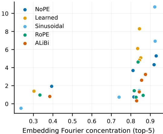
Uniform-attention ablation \Delta loss
