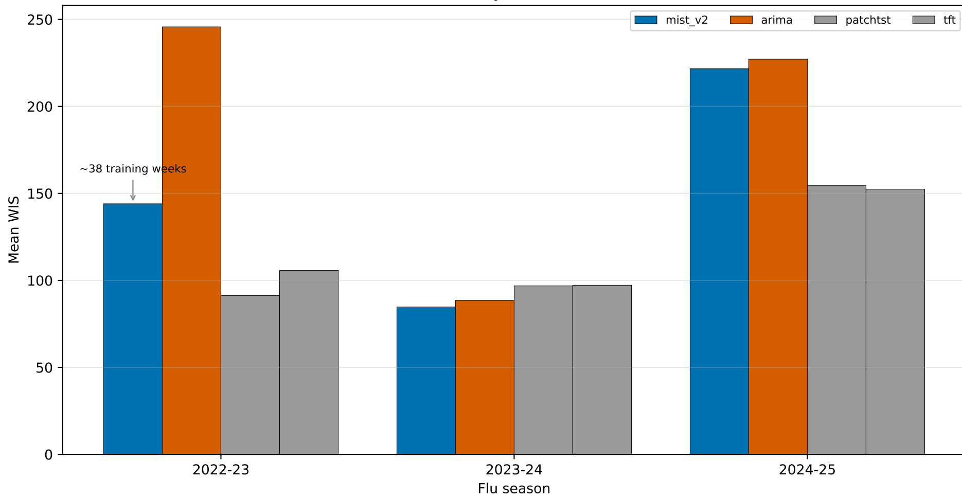
Cross-season WIS by model (lower is better)
