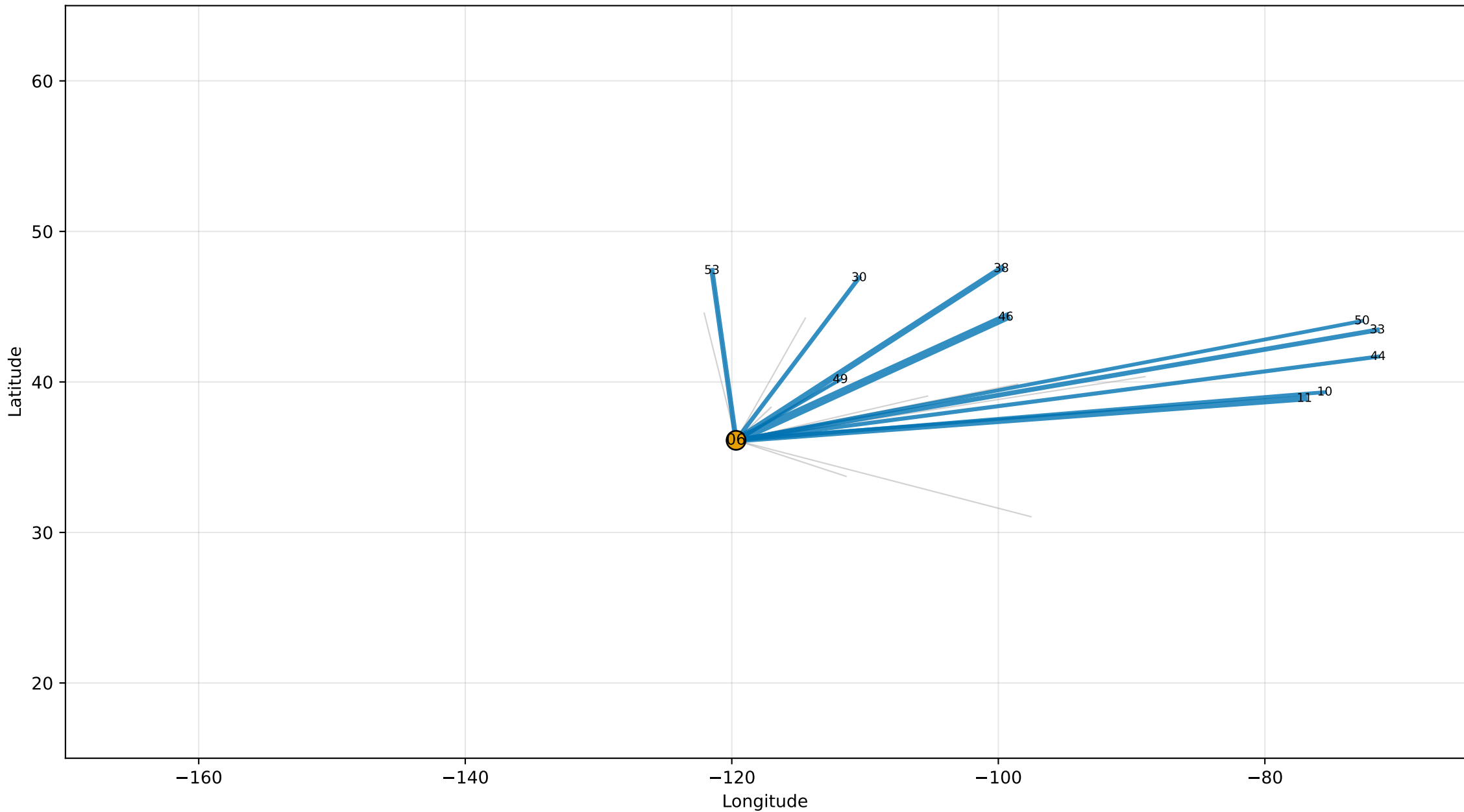
Learned spatial attention from 06 (blue) vs gravity mobility (grey), rising-phase week 2023-12-09
