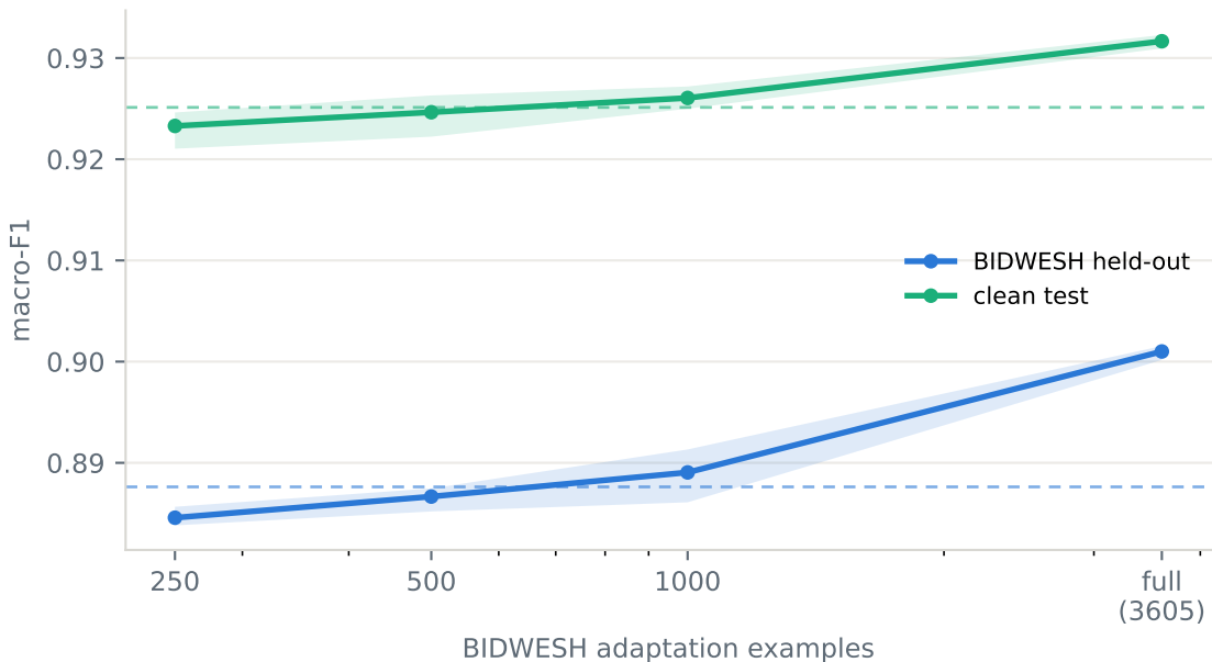
Few-shot dialect adaptation (dashed = no adaptation; band = seed min-max)
