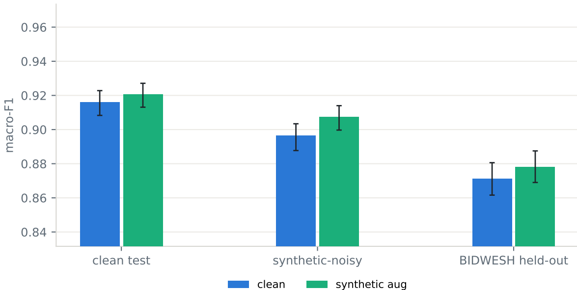
muril-base-cased: robustness by training variant (95% bootstrap CI)
