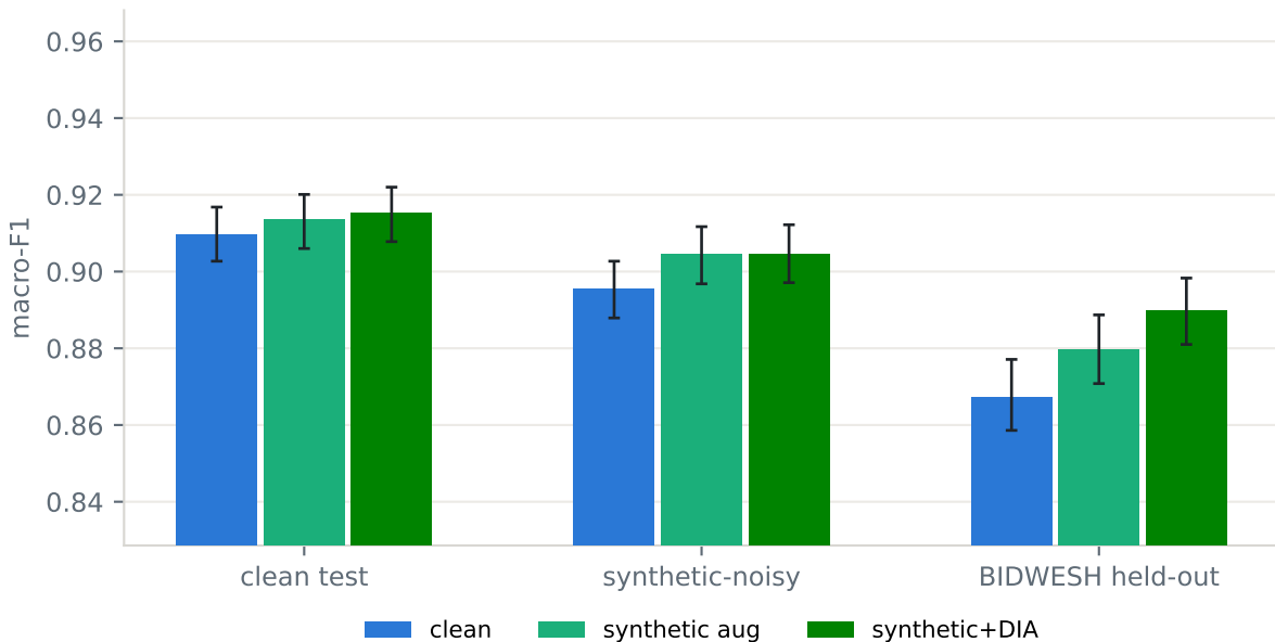
xlm-roberta-base: robustness by training variant (95% bootstrap CI)
