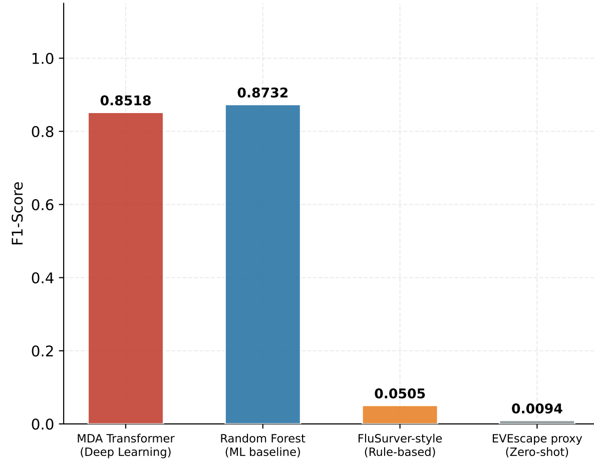
B F1-Score Comparison
