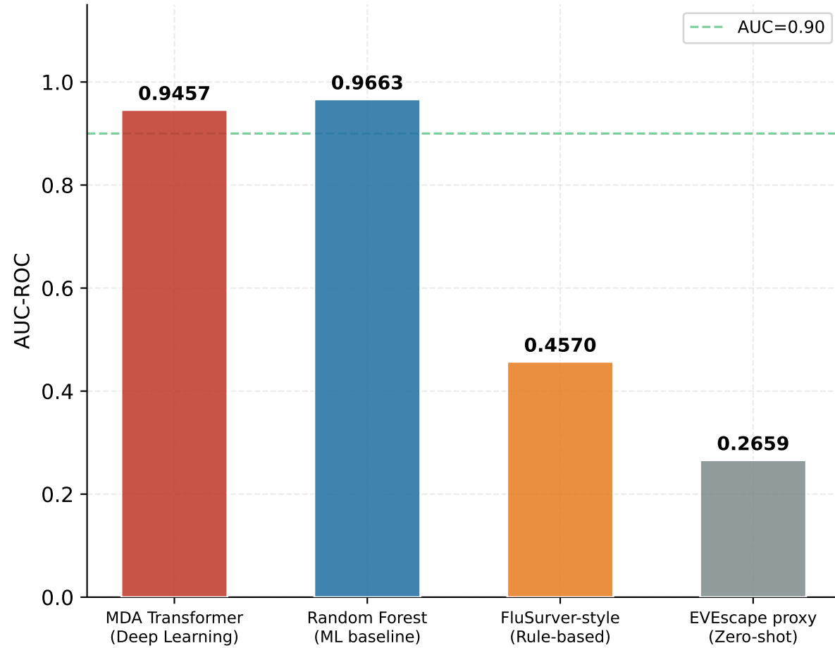
A AUC-ROC Comparison
