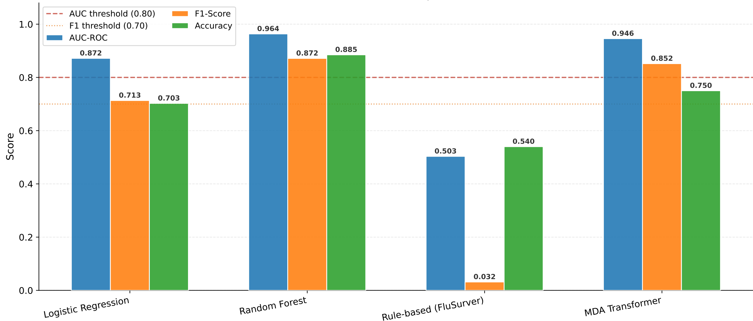
Figure 5. Performance comparison of drift prediction models on held-out test set ( n=400 mutations).
