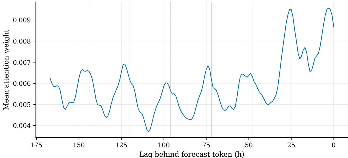
Forecast-token attention by lag (mean over layers/heads/windows)
