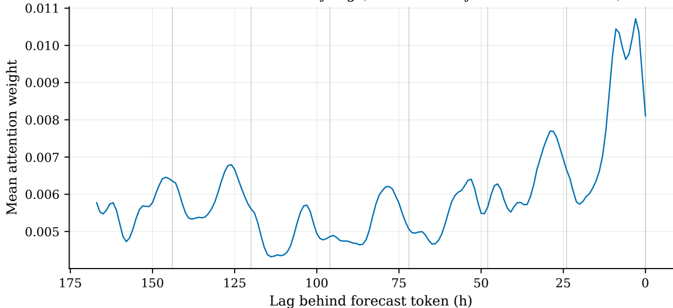
Forecast-token attention by lag (mean over layers/heads/windows)
