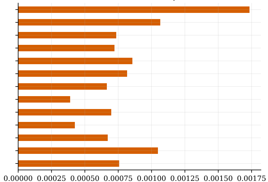
Gradient saliency
