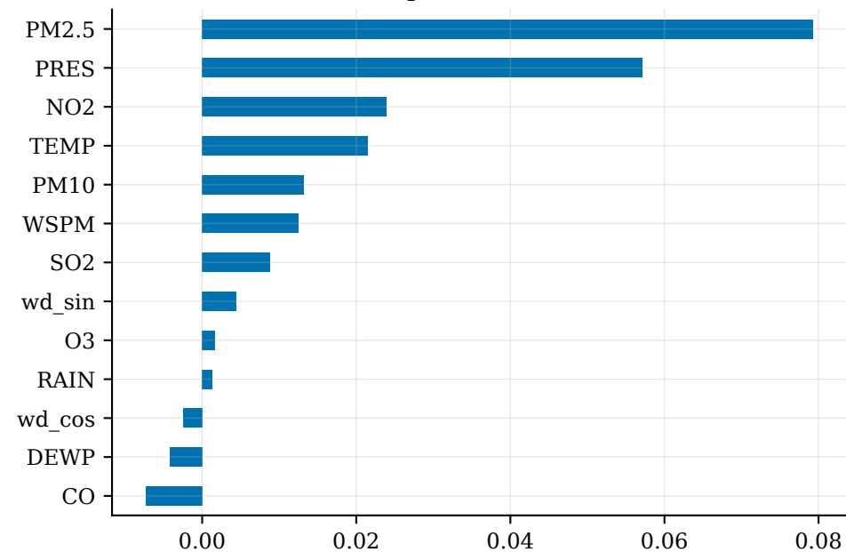
Permutation importance ( \Delta RMSE, scaled)
