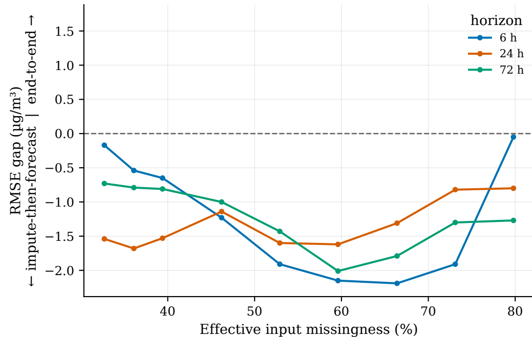
Cell-wise MCAR
