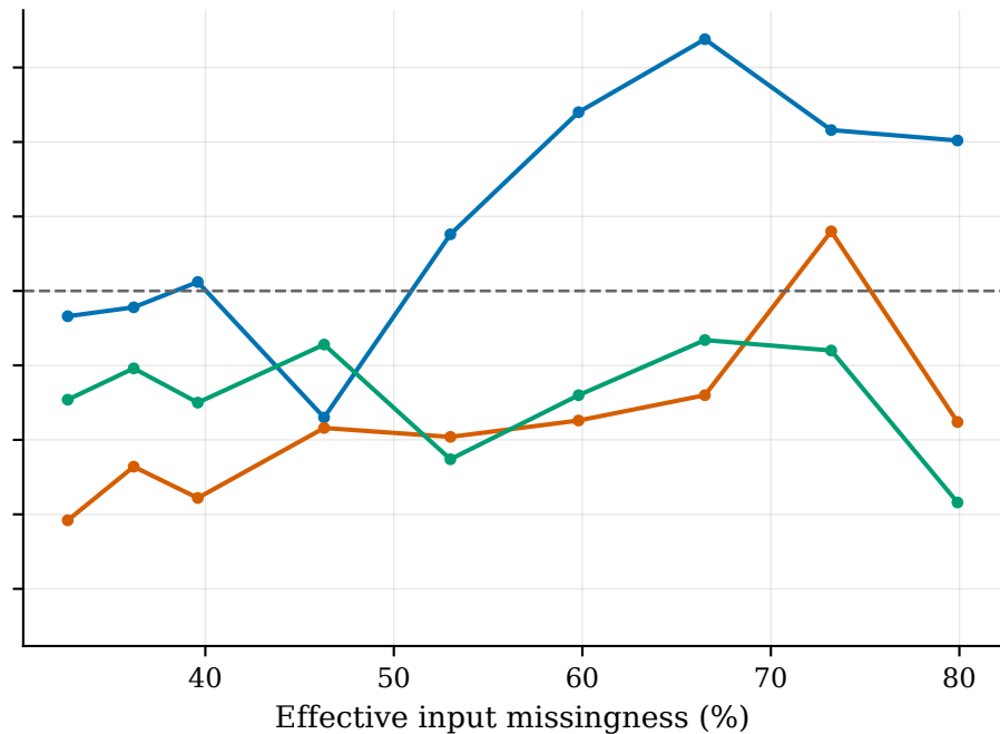
Station-outage blocks
