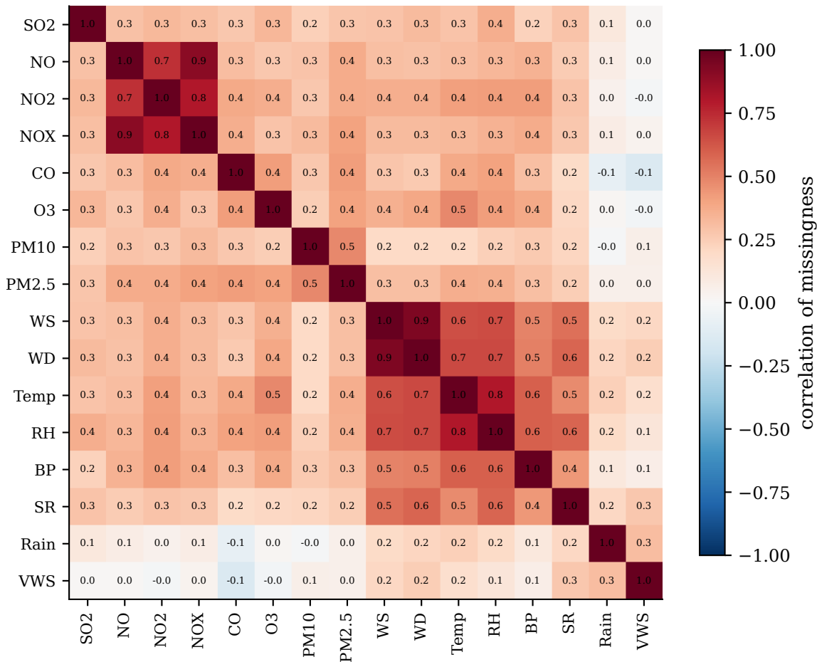
Co-missingness correlation matrix
