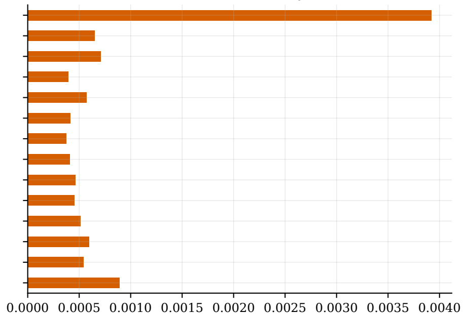
Gradient saliency
