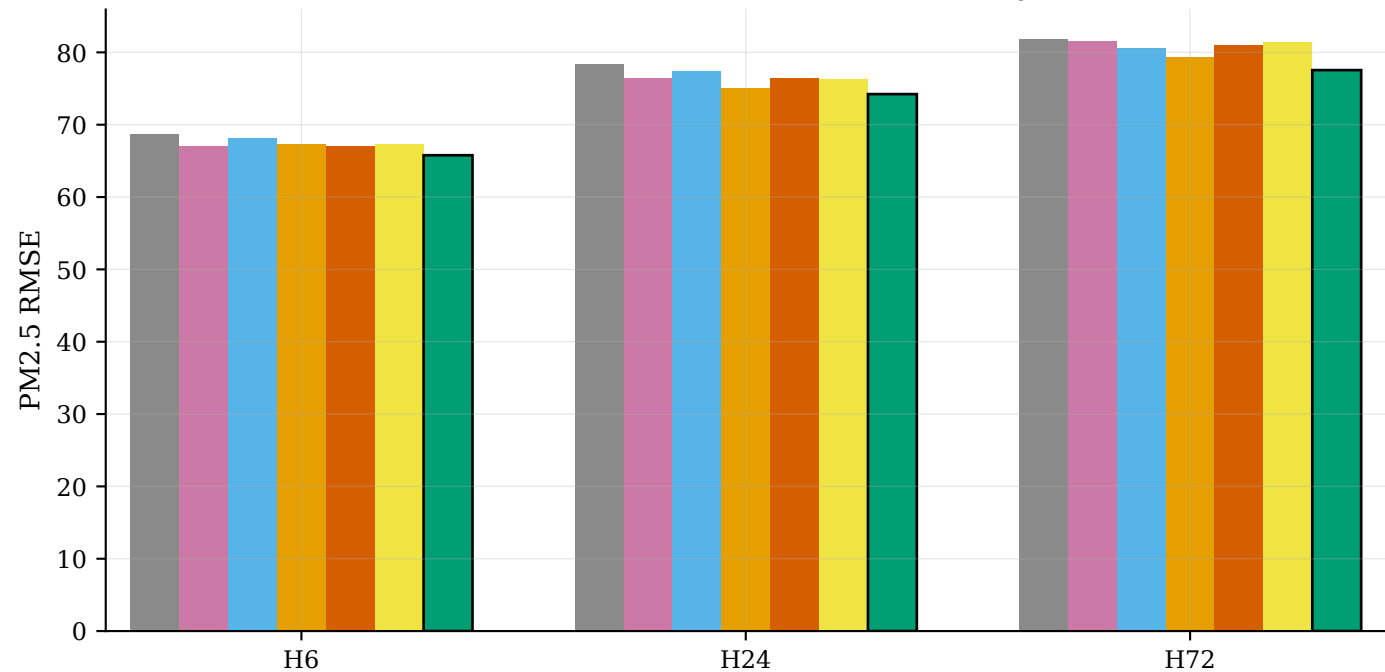
Final validation-calibrated MAT ensemble vs key baselines
