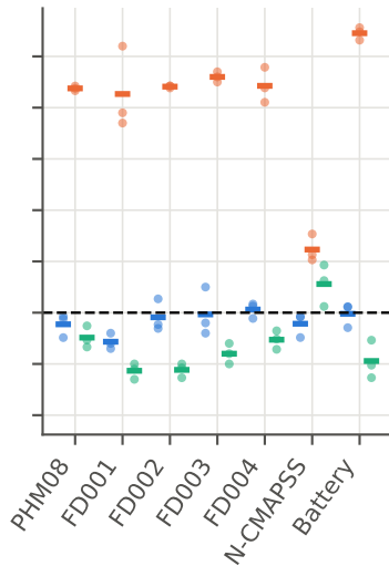
nominal \alpha = 0.20
