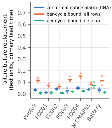
nominal \alpha = 0.05
