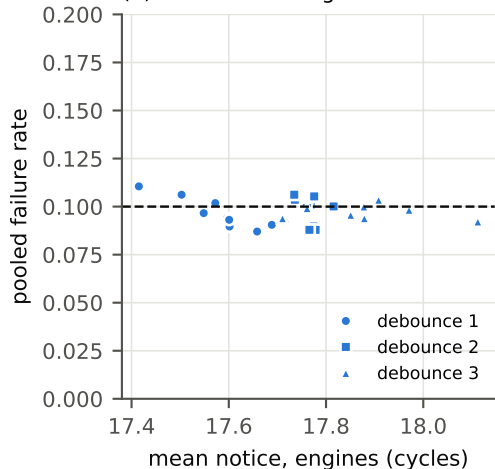
(b) 27 alarm settings of the GBM signal
