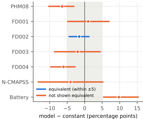
(a) window score difference, Tango 90% CI
