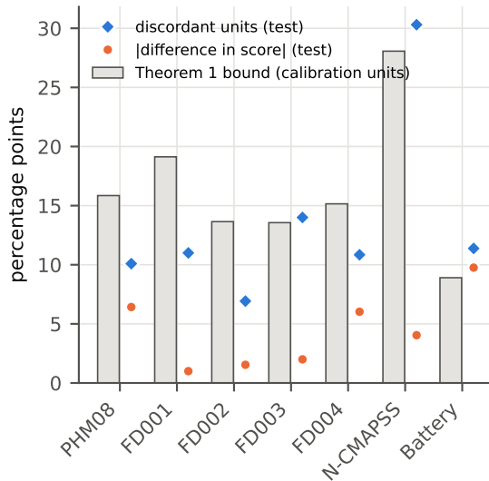
(b) bound vs realised discordance
