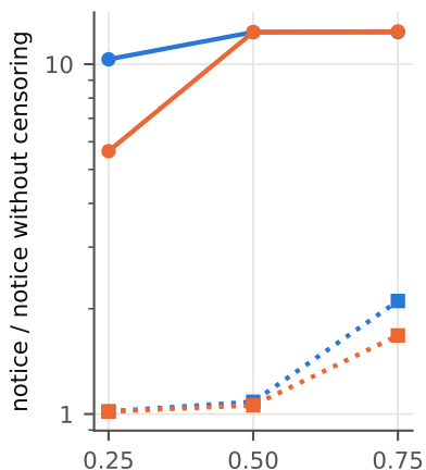
(b) notice vs. no censoring
