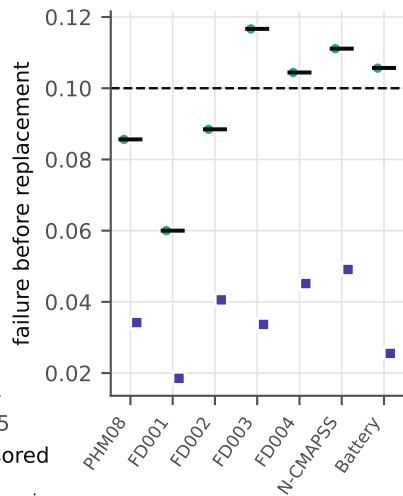
(c) history under an earlier alarm
