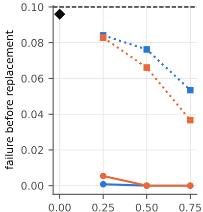
(a) validity ( \alpha = 0.10 )
