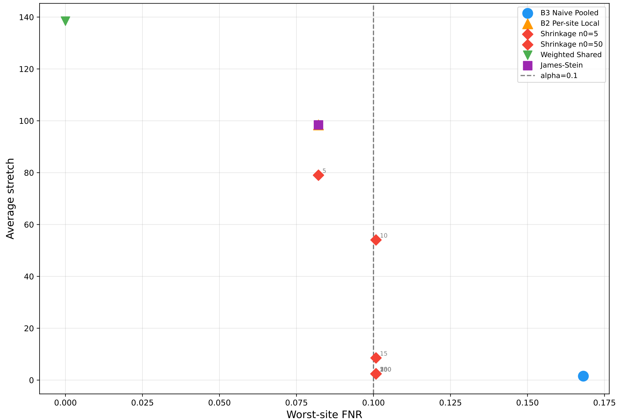
Pareto Frontier: Coverage vs Set Size FeTS-2022 REAL 23 Institutions (n=1251)
