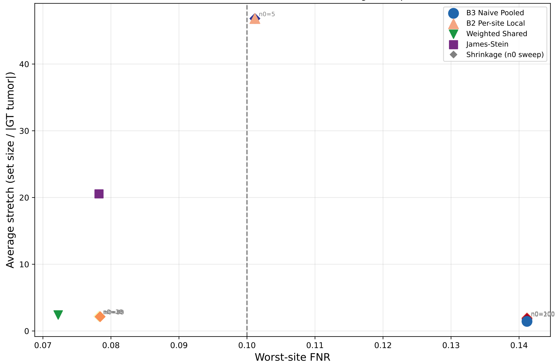
Pareto Frontier: Coverage vs Prediction Set Size (lower-left = better; ideal method is bottom-right of alpha line)
