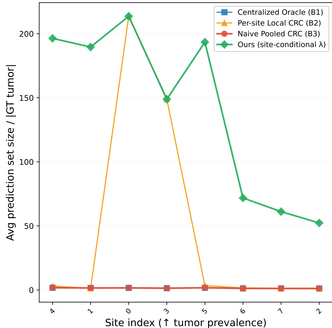
Per-site Prediction Set Size
