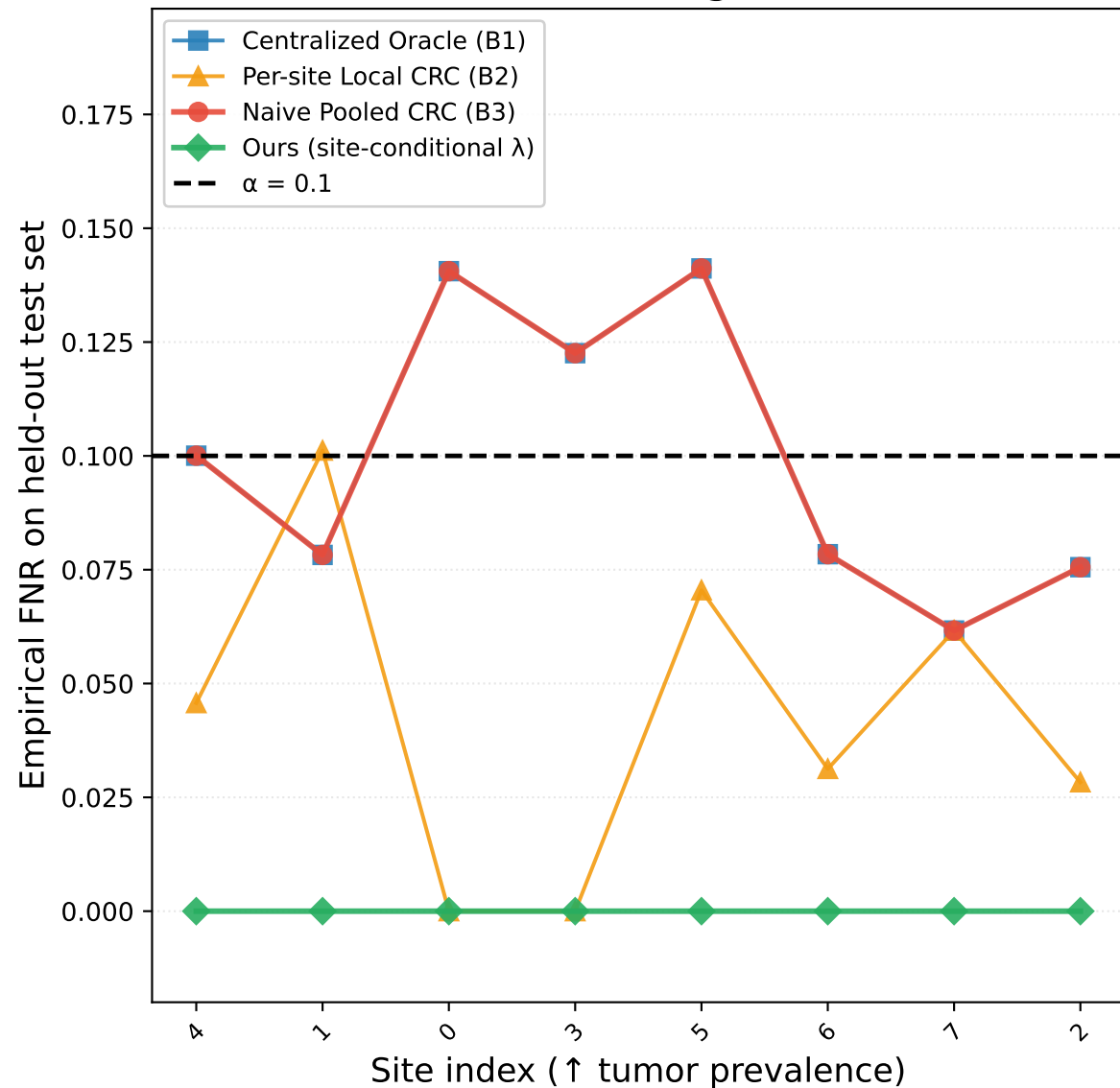
Per-site Coverage (FNR)
