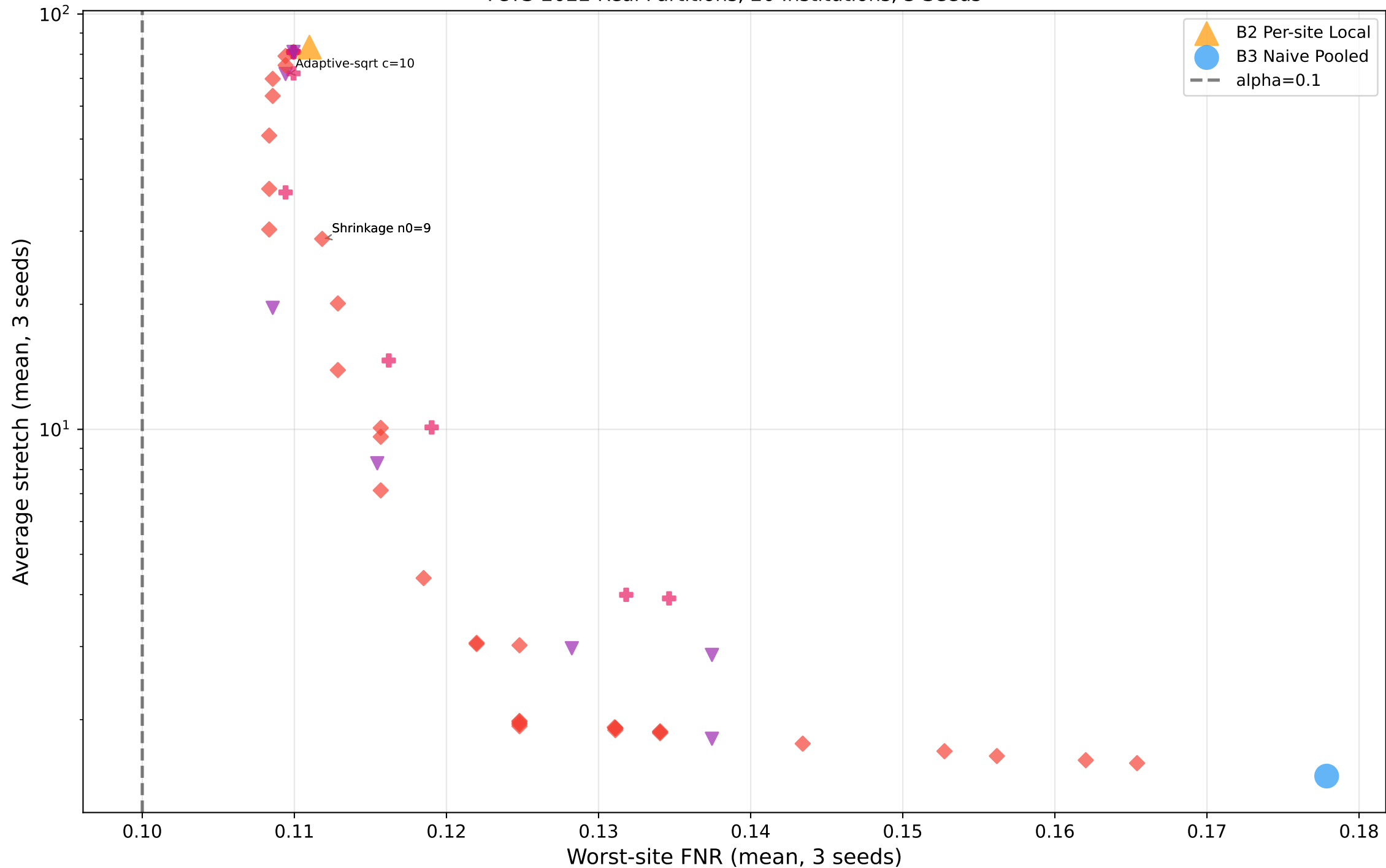
Pareto Frontier: Coverage vs Set Size FeTS-2022 Real Partitions, 20 Institutions, 3 Seeds
