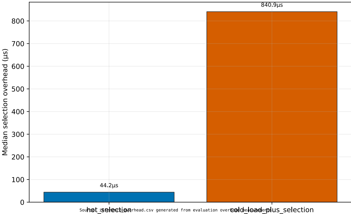
Inference overhead for AutoSBD selection
