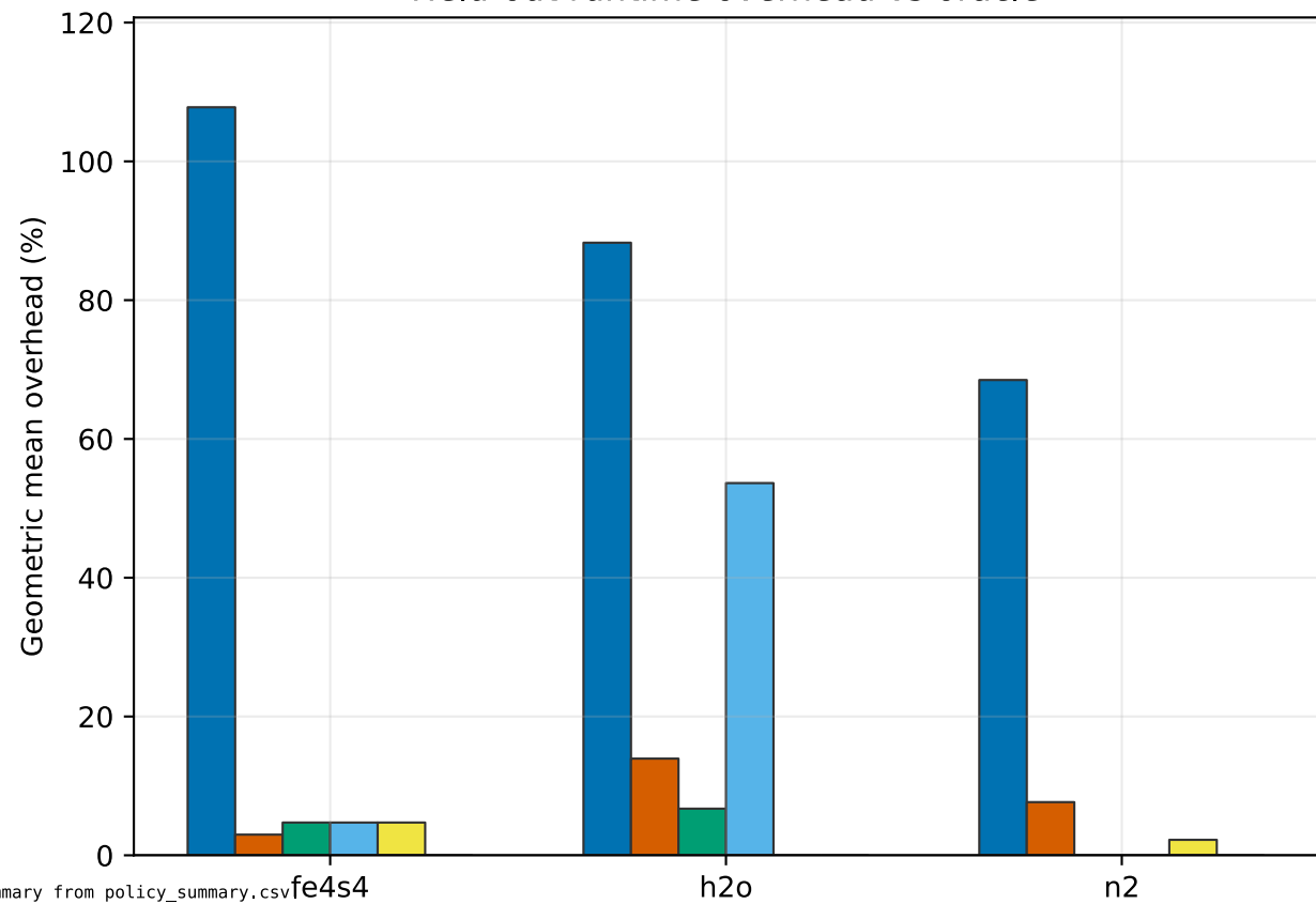
Held-out runtime overhead vs oracle
