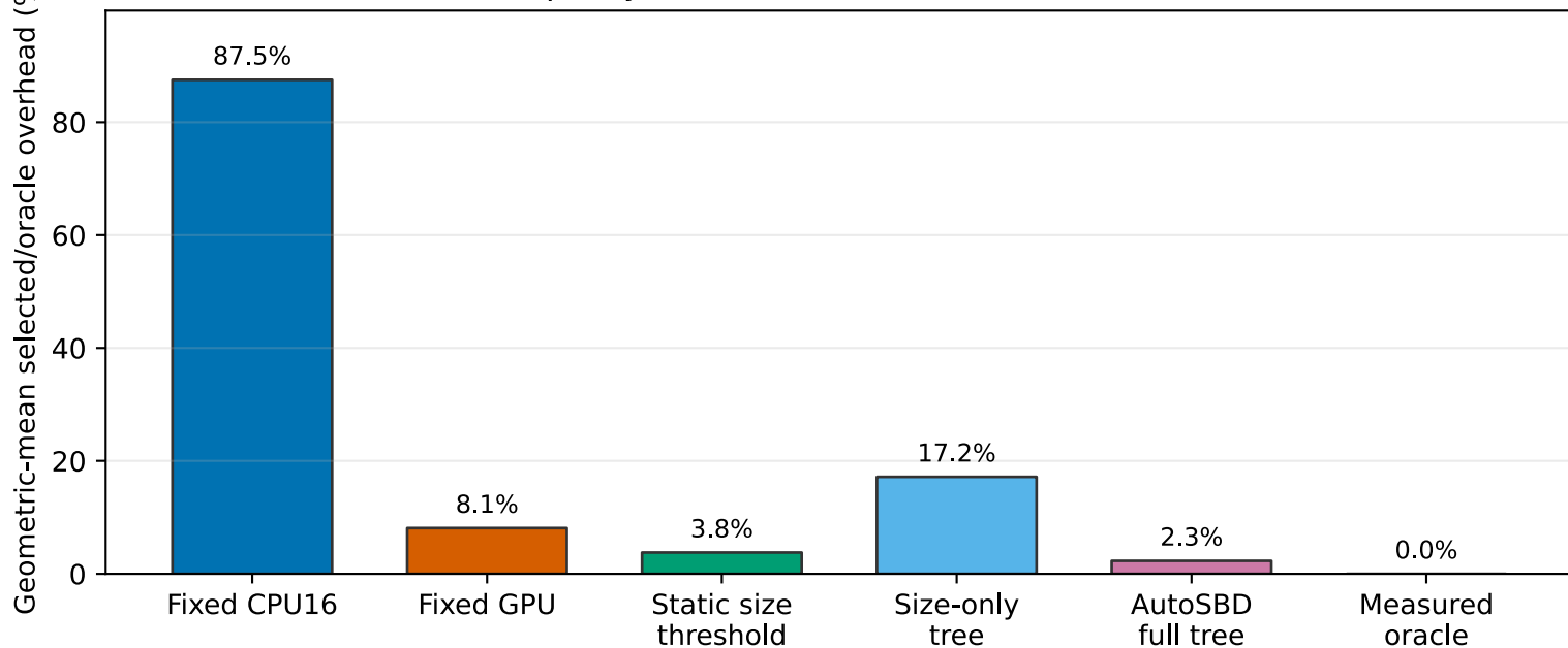
Held-out policy runtime overhead vs measured oracle
