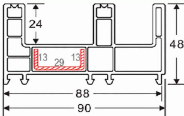
90 Sliding Frame
