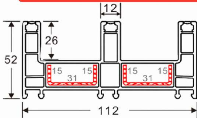
112 Sliding Frame
