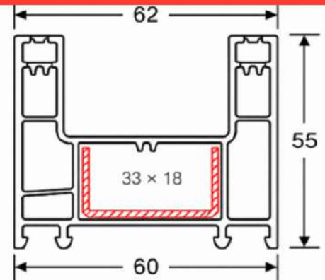
60 Double Sliding Frame A
