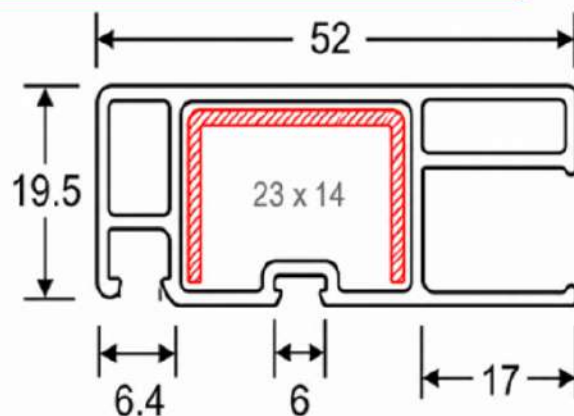
Screen Sash A2
