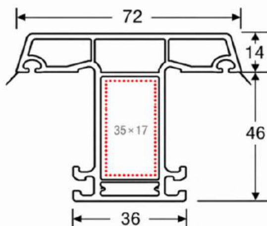
60 Mullion C
