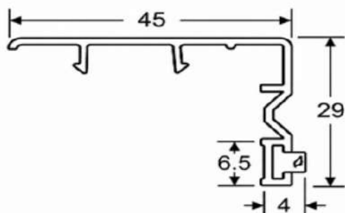
88 Sliding Sash Cover
