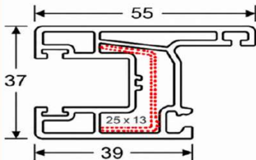
80 Sliding Sash H
