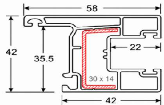
88 Sliding Sash E
