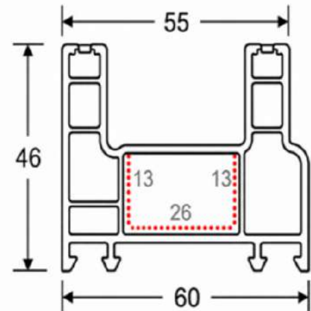
60 Double Sliding Frame B
