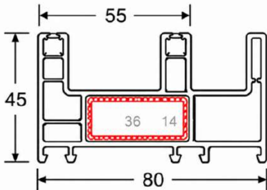
80 Sliding Frame 45-2
