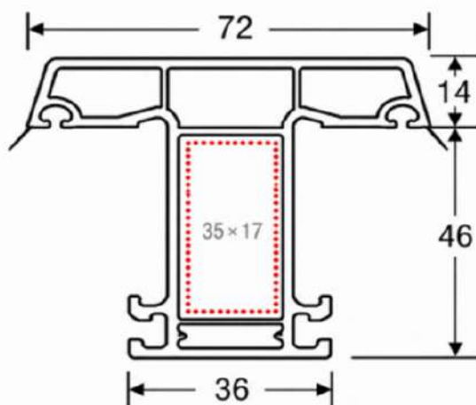
60 Mullion C
