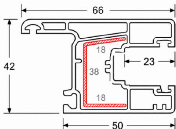
88 Sliding Sash 2
