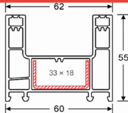
60 Double Sliding Frame A
