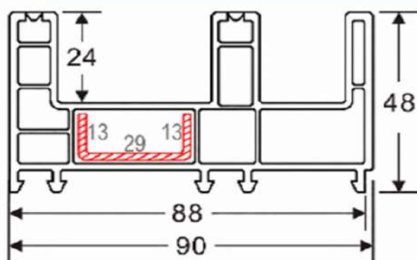
90 Sliding Frame
