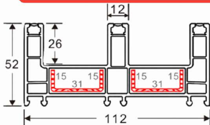
112 Sliding Frame
