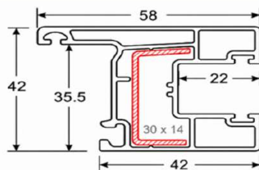
88 Sliding Sash E
