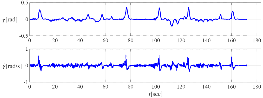
Figure 7: Steering Angle & Rate of Closed-Loop Simulation
