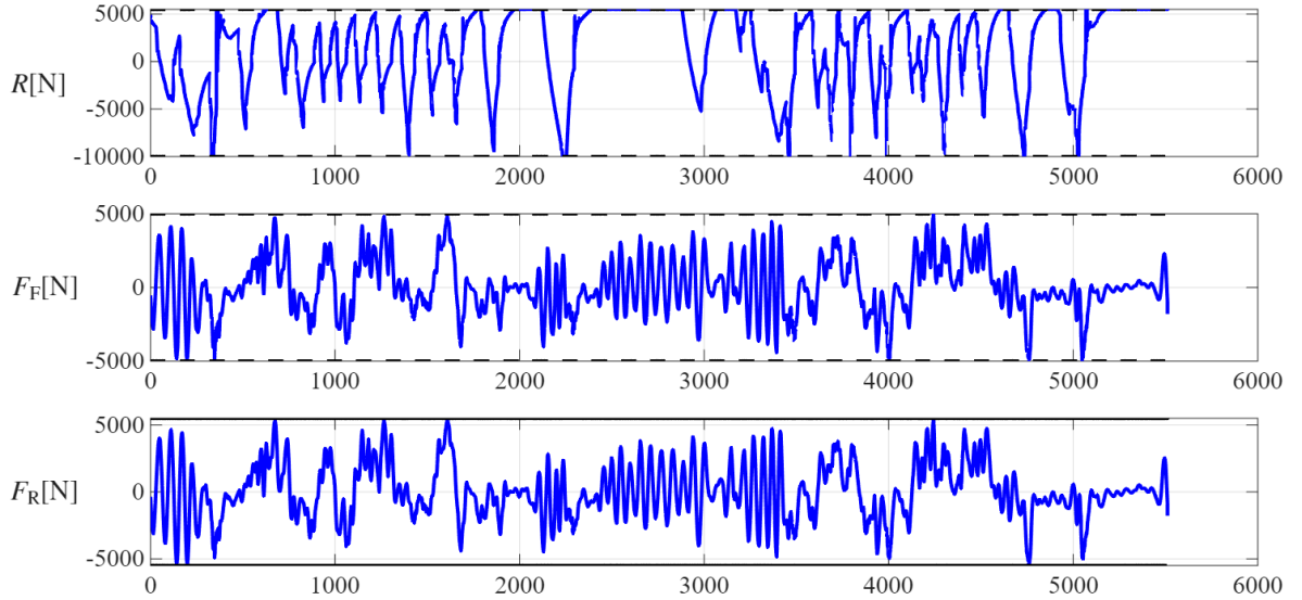
Figure 6: Force Plots of Closed-Loop Simulation
