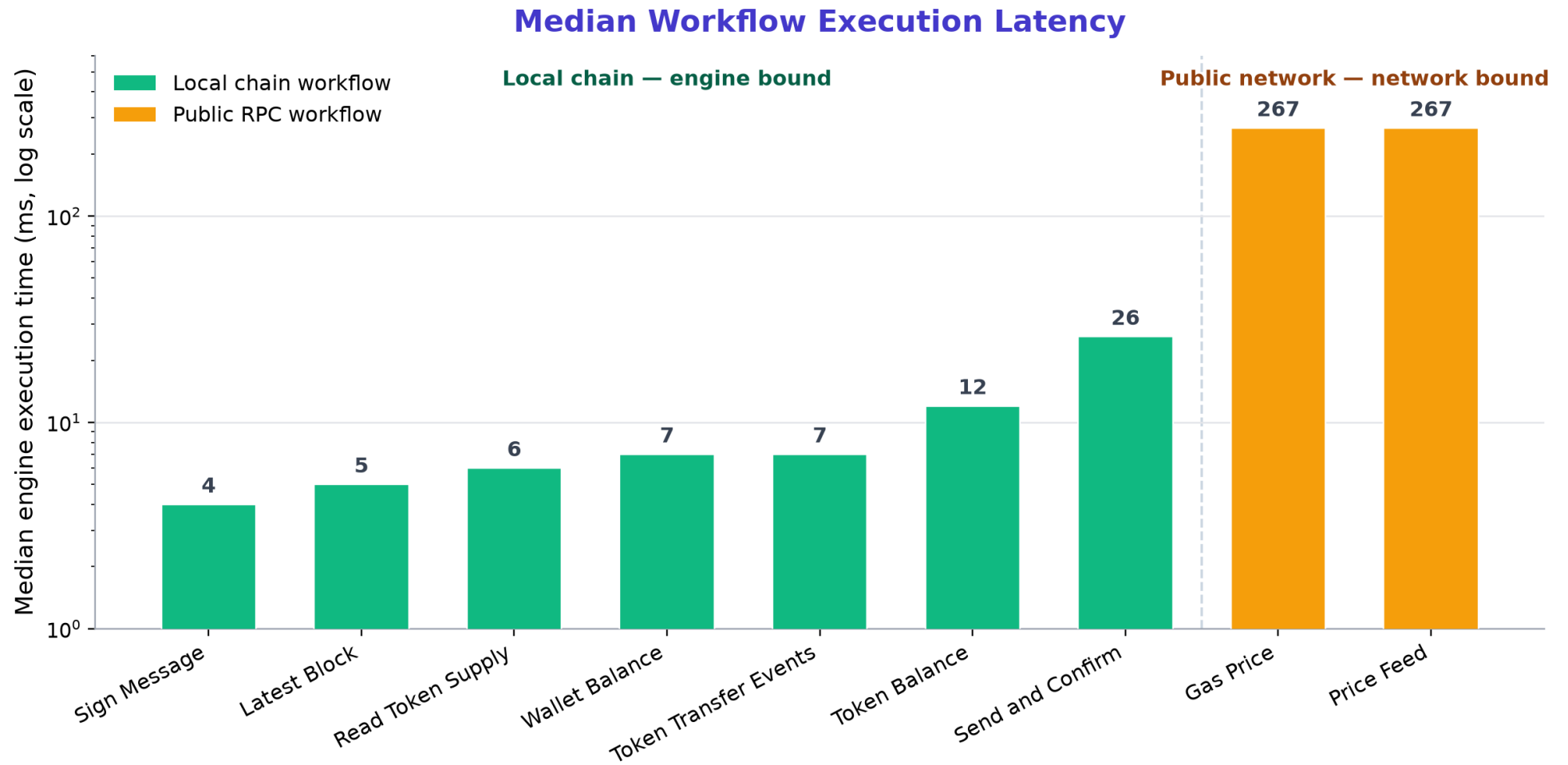
Fig 6.1 Median Workflow Execution Latency
