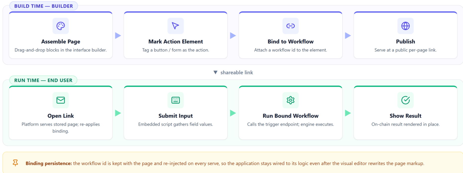
Fig 3.6 Interface Binding and Hosting Flow
