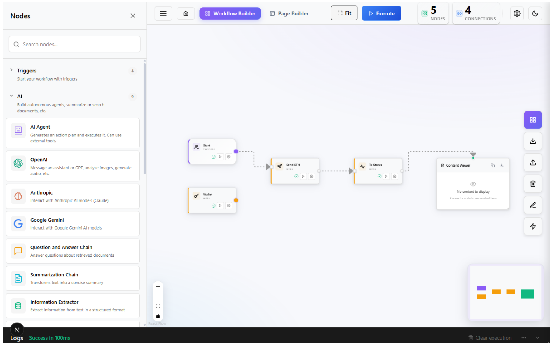
Fig A.2 Visual Workflow Builder Interface
