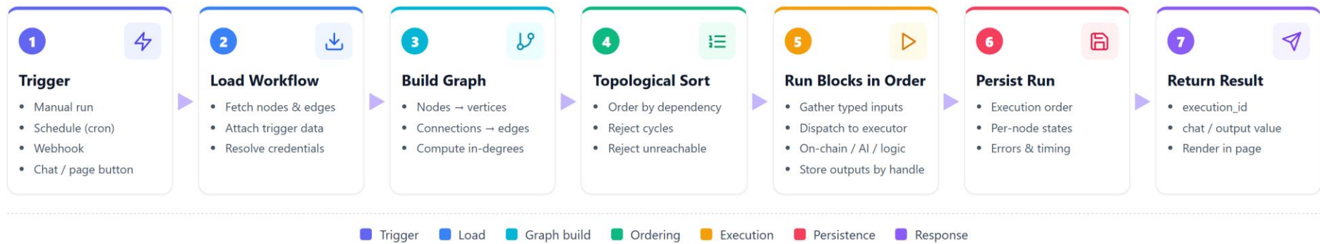
Fig 3.4 Workflow Execution Model
