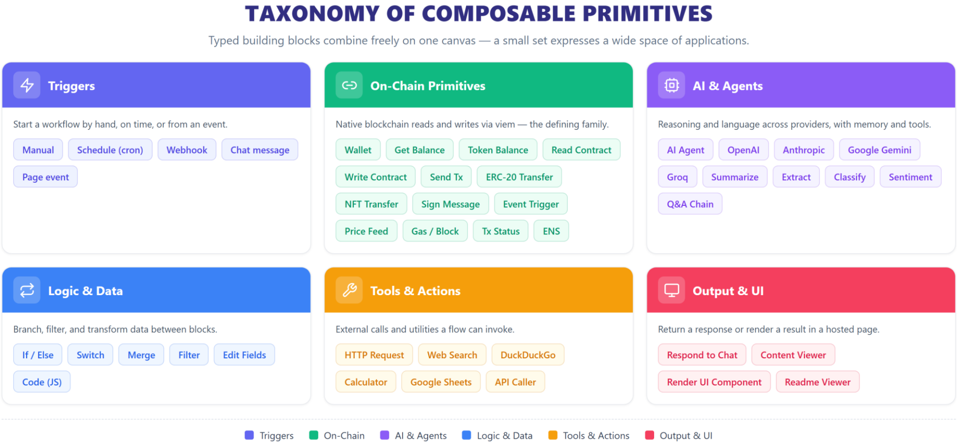
Fig 3.5 Taxonomy of Composable Primitives
