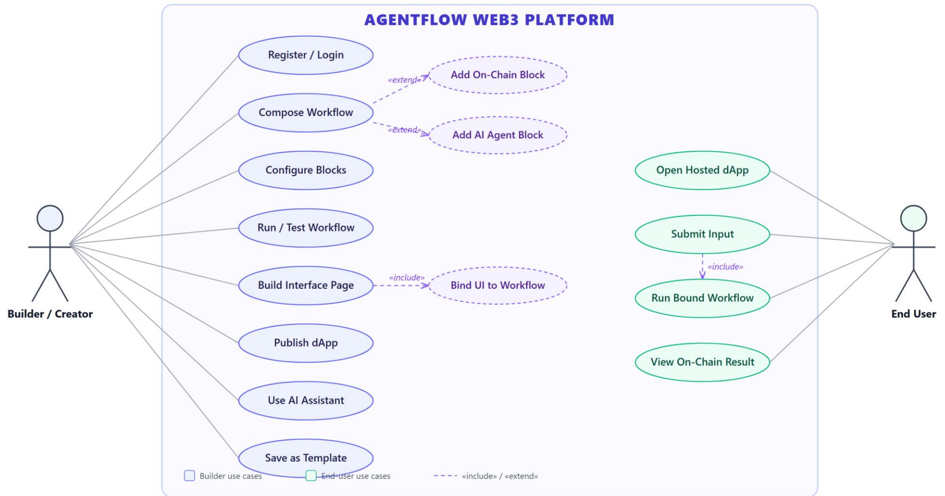
Fig 3.2 Use Case Diagram
