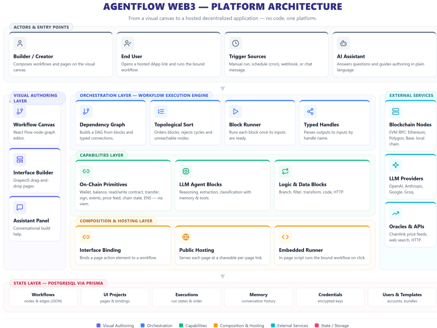
Fig 3.1 AgentFlow Web3 System Architecture
