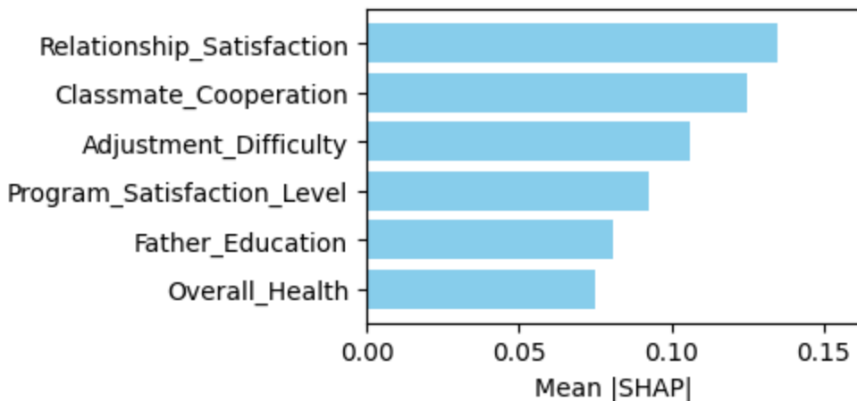
XGBoost
