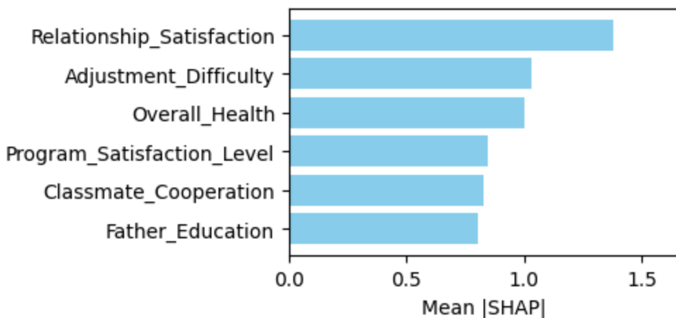
XGBoost
