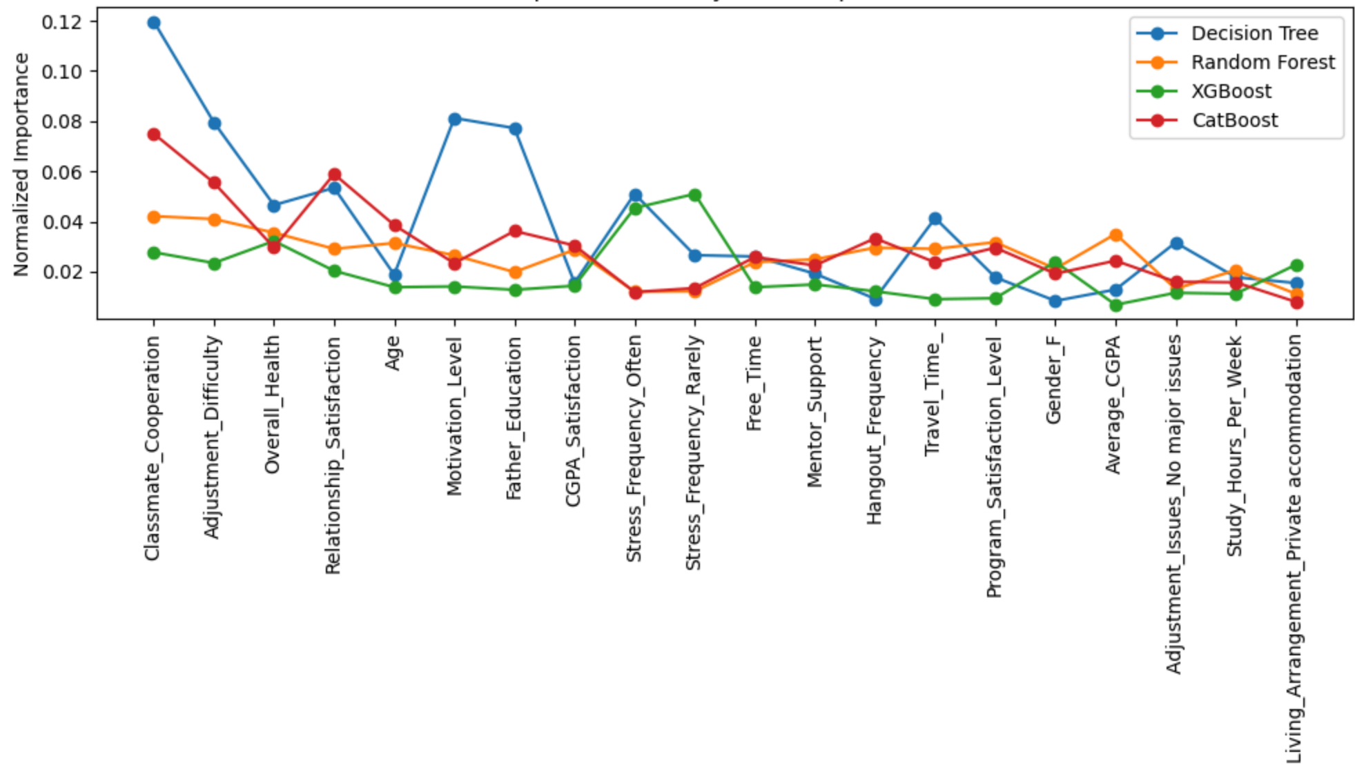
Top 20 Features by Model Importance
