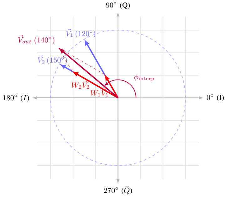
Fig. 3. Phasor construction for the CMPI. Blue: boundary phasors \vec{V}_1 ( 120^\circ ) and \vec{V}_2 ( 150^\circ ). Red: weighted components W_1\vec{V}_1 , W_2\vec{V}_2 . Purple: resultant interpolated phase at 140^\circ . The weight ratio W_2/W_1 = \sin(\phi - \phi_1)/\sin(\phi_2 - \phi) follows from the sine rule.
