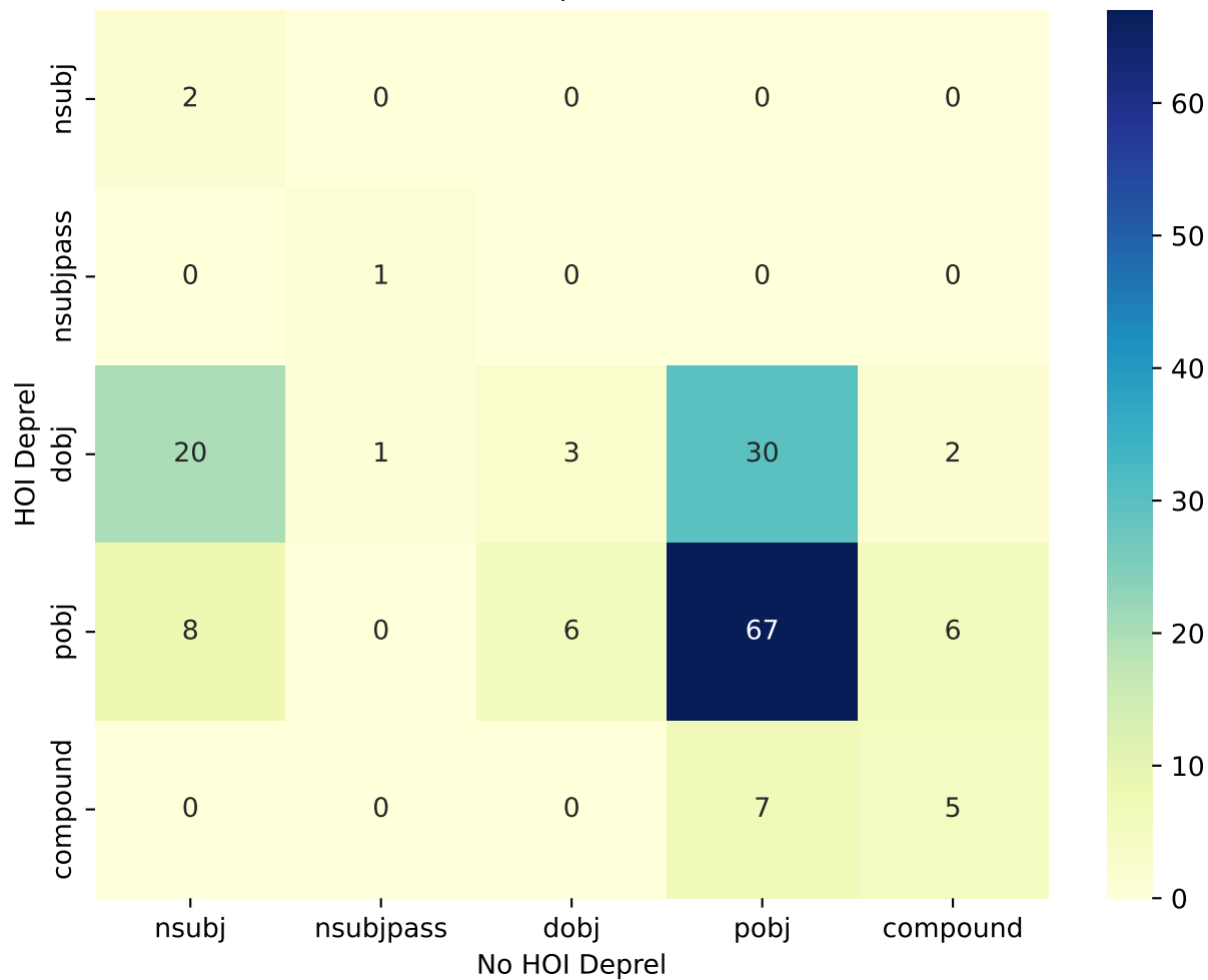
HOI vs no HOI Deprel Co-occurrence
