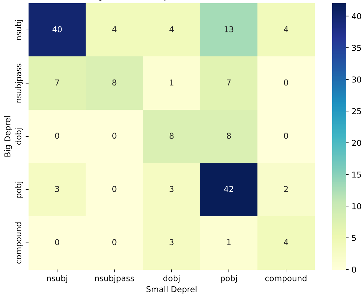
Big vs Small Deprel Co-occurrence
