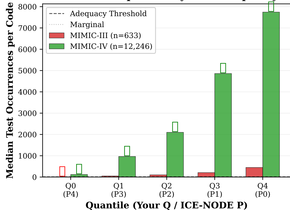
Test Set Sample Size by Code Frequency
