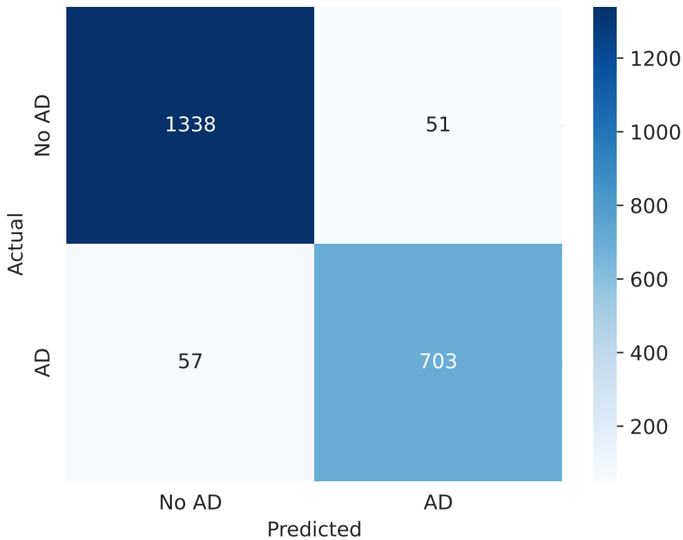
CALiBRE-AD Confusion Matrix (thr=0.32)
