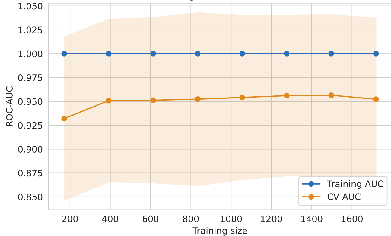
Learning Curve (Full track)
