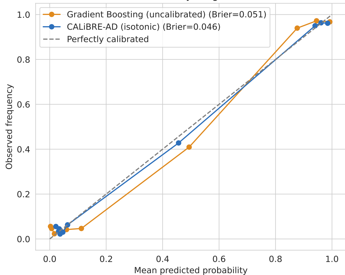
Reliability Diagram
