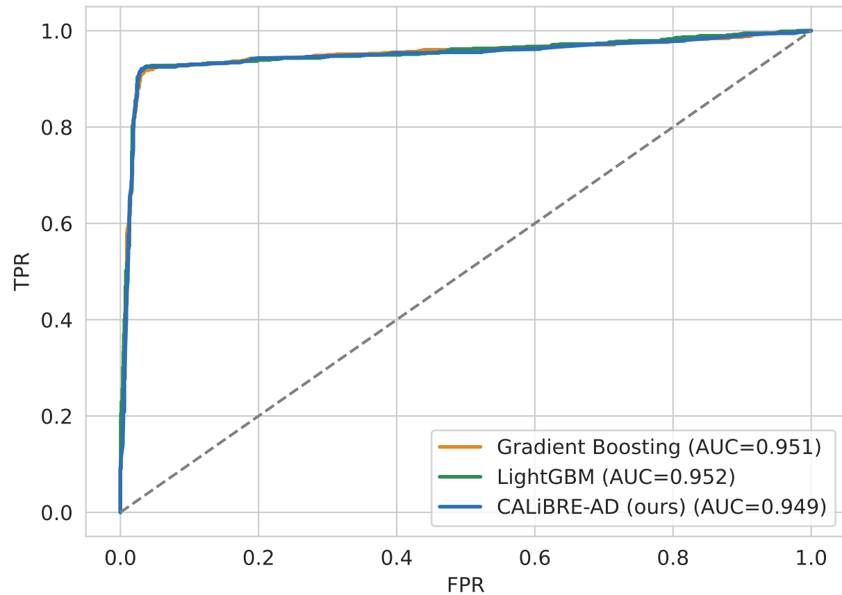
ROC (Full track)
