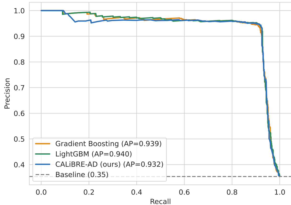
Precision-Recall (Full track)
