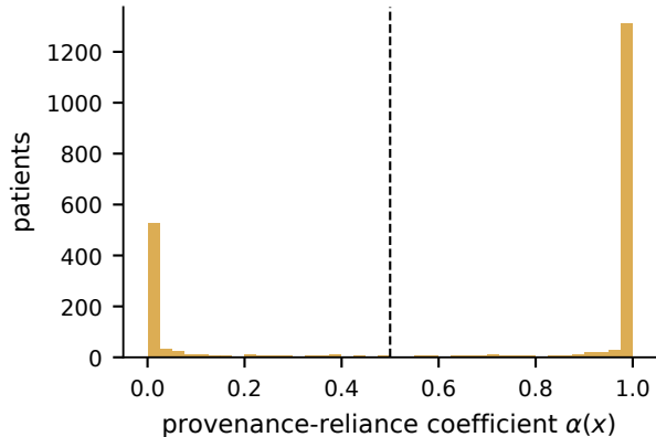
routing is crisp, not diffuse
