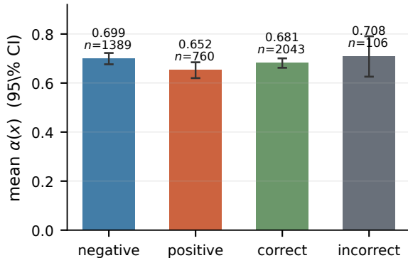
reliance by outcome group
