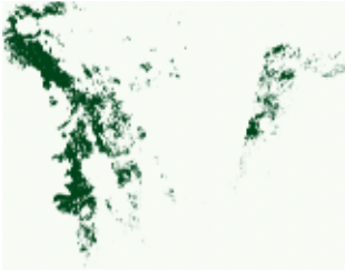
Optical MNDWI (total water)
