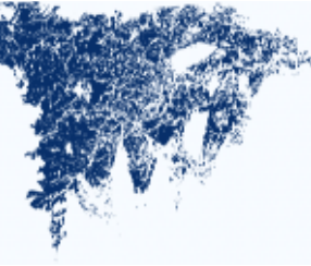
S1 flood (change-based)
