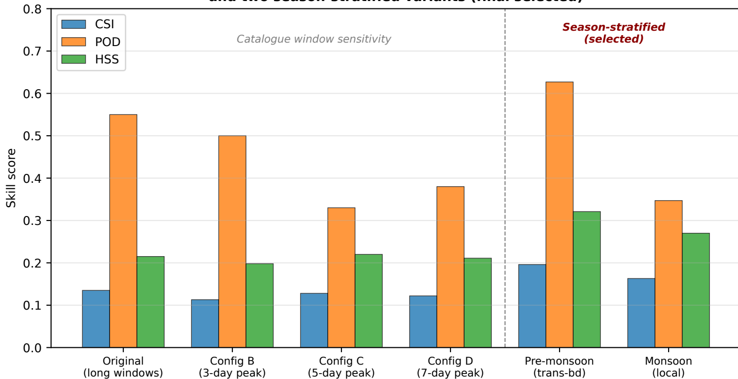
Figure S2. Robustness of triggers across four catalogue configurations and two season-stratified variants (final selected)
