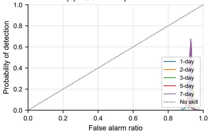
(c) ROC curves per window
